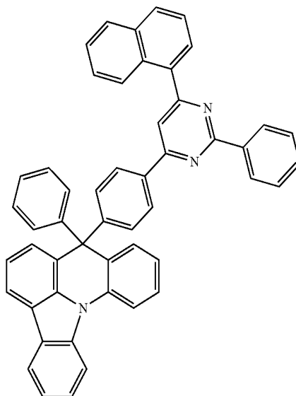
[Compound 40]
