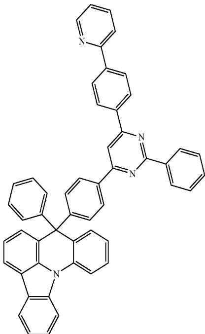
[Compound 33]
