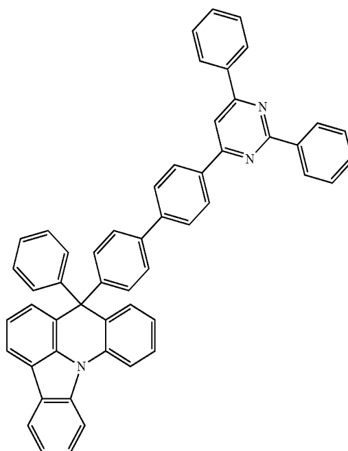
[Compound 36]
