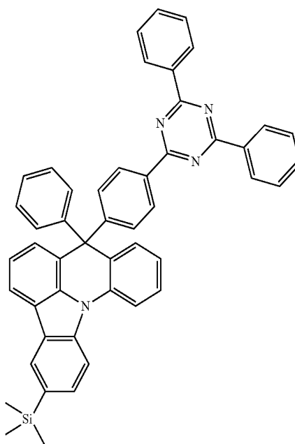
[Compound 109]
