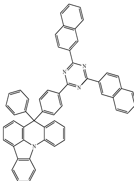
[Compound 13]
