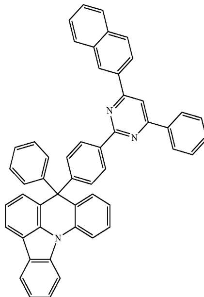
[Compound 59]
