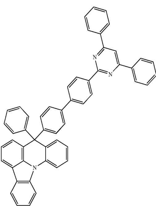
[Compound 54]
