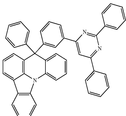
[Compound 44]
