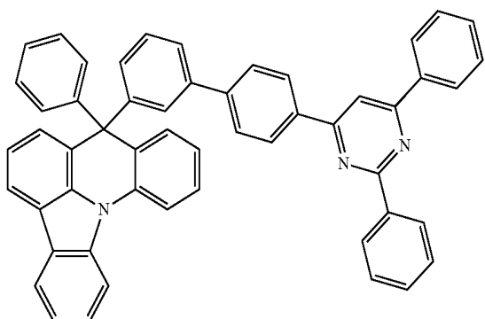
[Compound 39]
