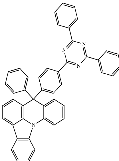
[Compound 28]
