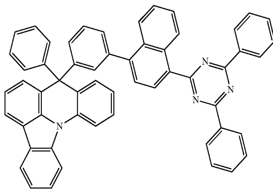
[Compound 18]
