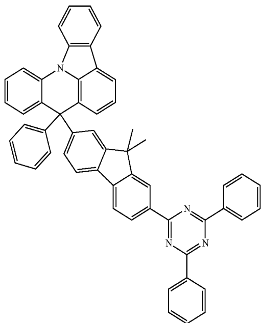
[Compound 25]
