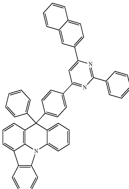
[Compound 41]
