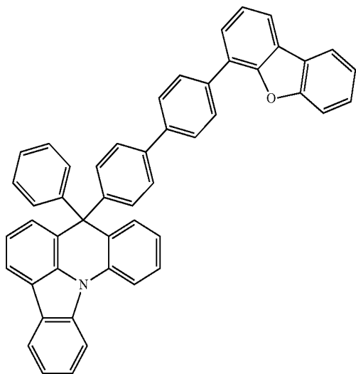
[Compound 79]
