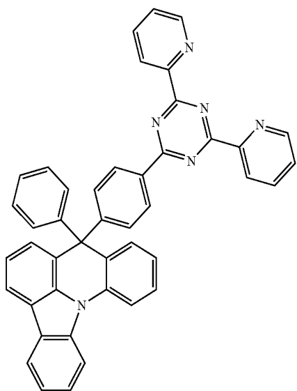
[Compound 16]
