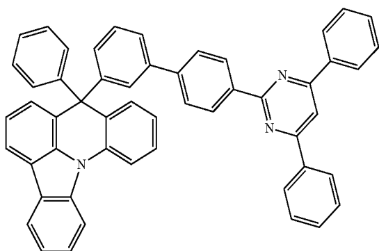
[Compound 57]
