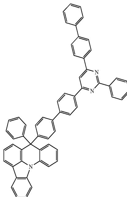
[Compound 38]
