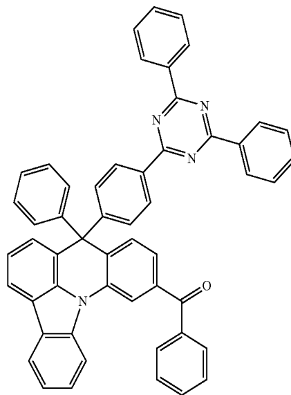
[Compound 112]
