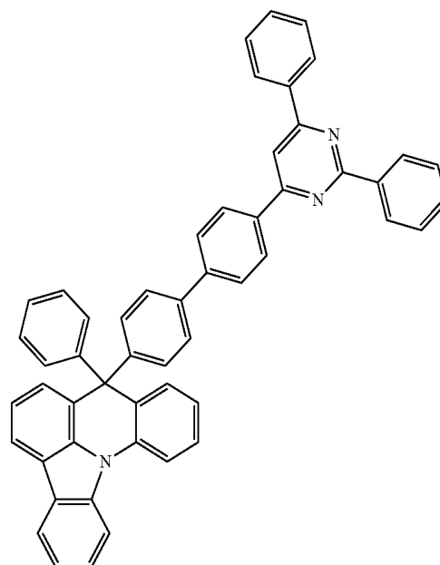
[Compound 37]
