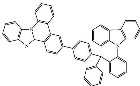
[Compound 8]
