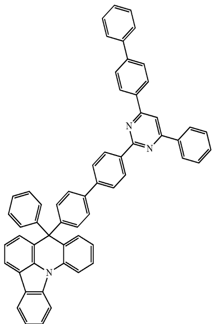
[Compound 56]
