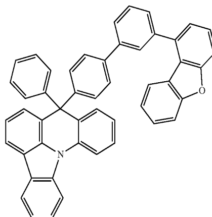
[Compound 83]
