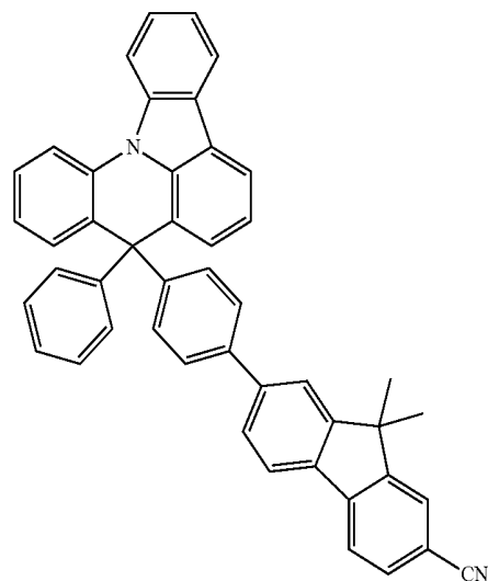
[Compound 92]
