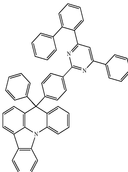
[Compound 50]
