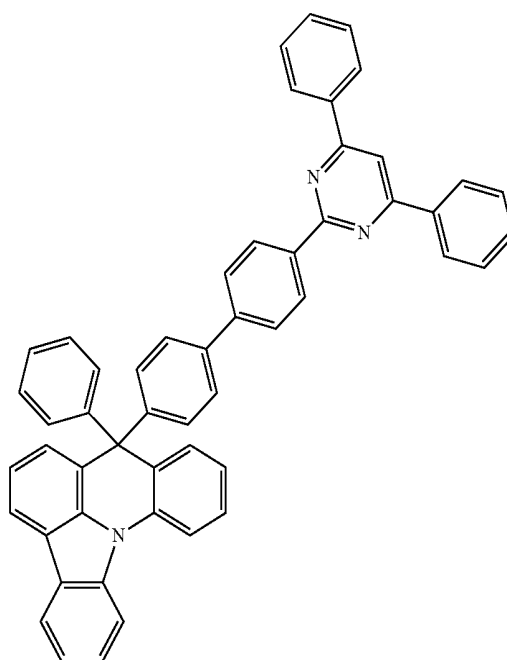
[Compound 53]
