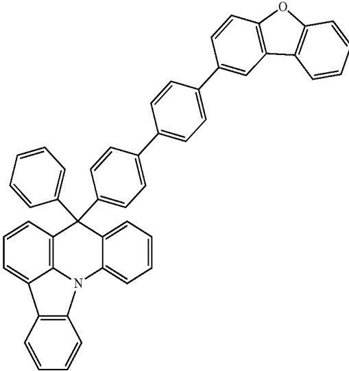
[Compound 77]
