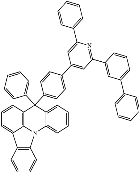
[Compound 74]
