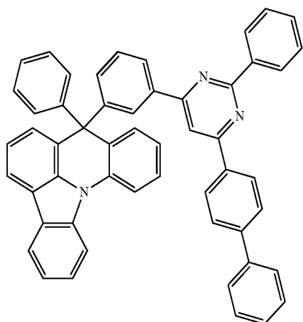
[Compound 45]
