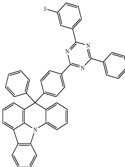
[Compound 27]
