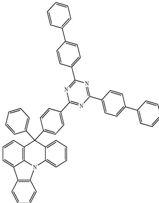
[Compound 5]
