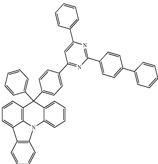
[Compound 30]
