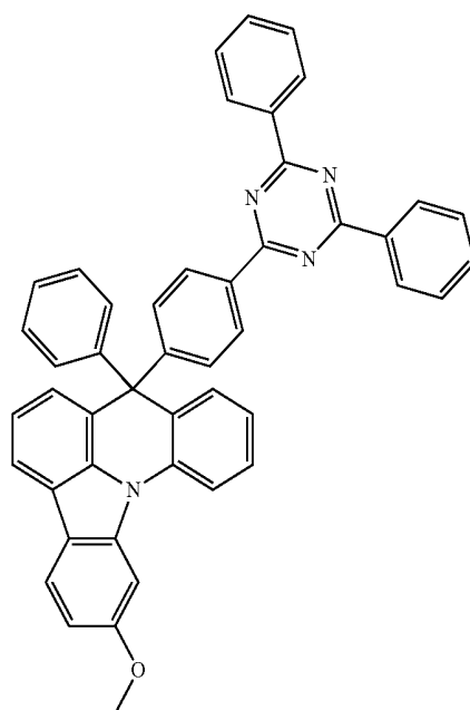
[Compound 110]
