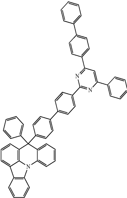
[Compound 55]
