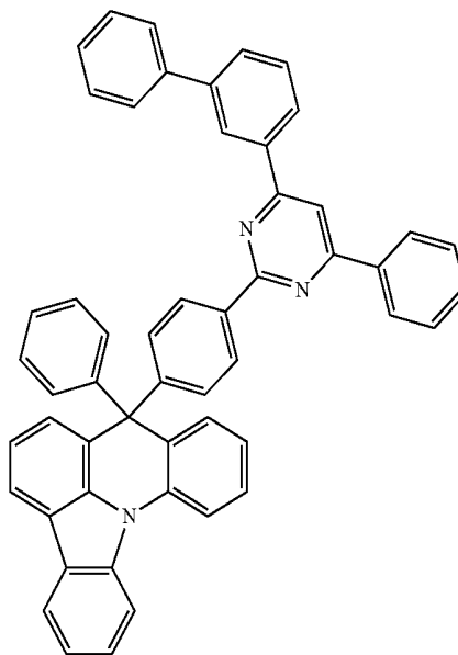
[Compound 49]
