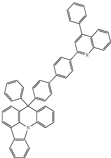
[Compound 101]
