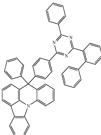
[Compound 4]
