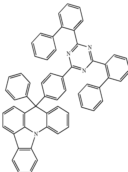
[Compound 7]
