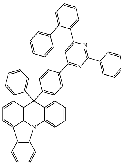
[Compound 32]
