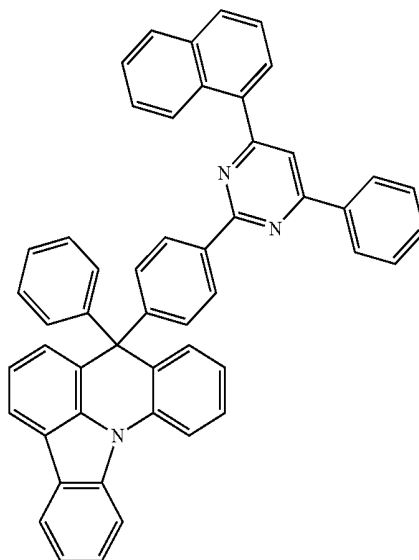
[Compound 58]
