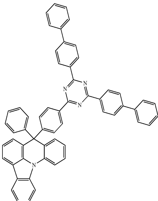
[Compound 5]
